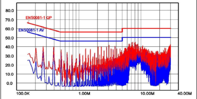
Typical Conducted Emmissions
