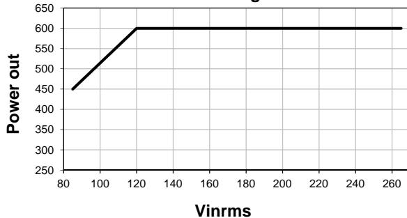
Line Derating
