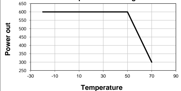
Temperature Derating
